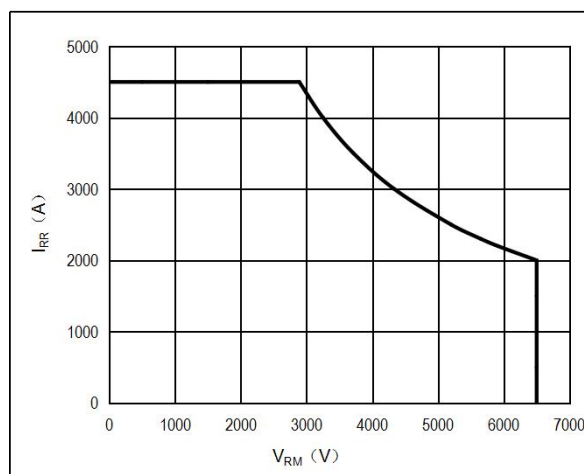
图8. 反向恢复安全工作区 (RRSOA) Fig.8 Reverse recovery safe operating area
